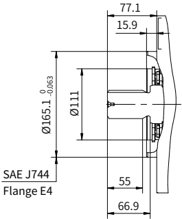
"E1" type spline shaft ANSI B92.1b 1 3/4 in 13T-8/16 DP
