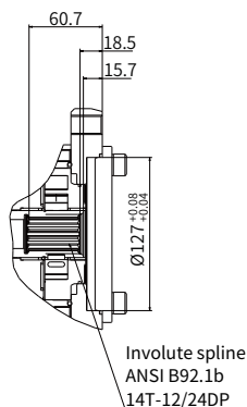
“C6” type through drive
