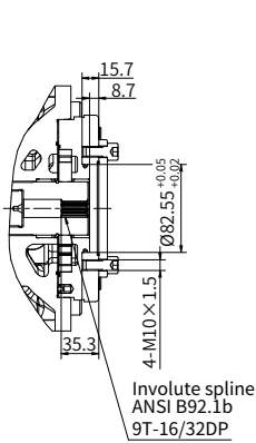
"A1" type through drive
