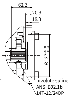
“C2” type through drive
