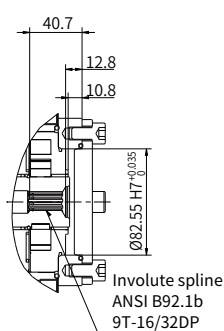
“A1” type through drive
