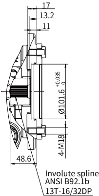
"B1" type through drive
