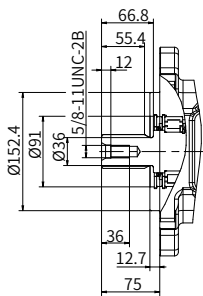
“D1” type spline shaft ANSI B92.1b 1 3/4 in 13T 8/16 DP
