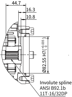
"A2" type through drive
