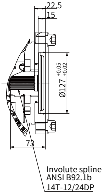
"CC" type through drive
