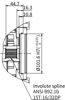
"B3" type through drive
