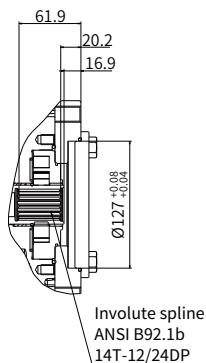
“CC” type through drive
